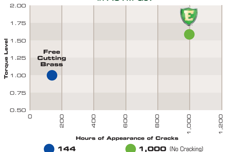
Stress Corrosion Cracking Performance in ASTM G37
